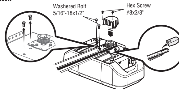
Washed Bolt 5/16"-18x1/2" (Mounted in the garage door opener) Model 8550W (2) Model 8557W (1)
